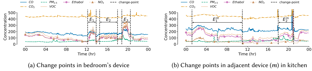
Fig. 4. Detected time segments from the change points computed using the KLCPD algorithm for two adjacent devices in the bedroom and kitchen. The event E_2^m in the kitchen's device and E_3 in the bedroom's device are associated with significant time overlap.
