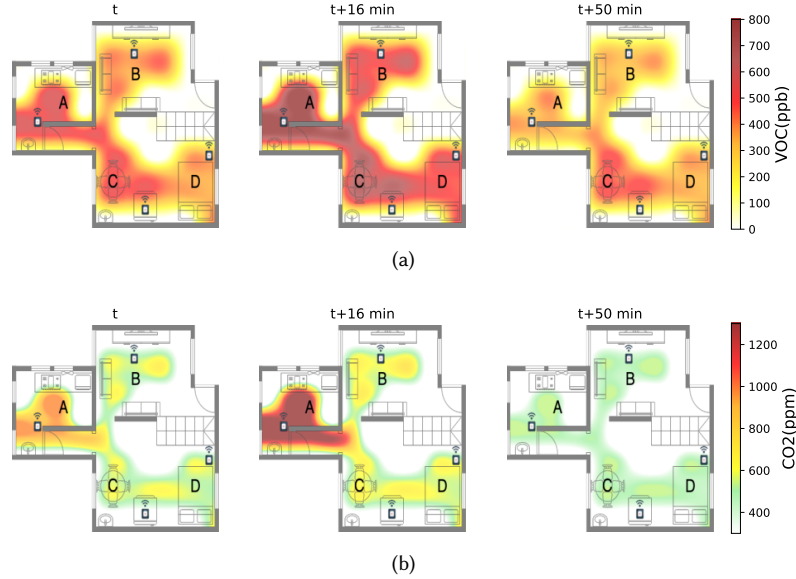
Fig. 16. Spatiotemporal spread of – (a) VOC, and (b) CO 2 from the kitchen (A) in Household H2. The cooking starts at t and ends at t+30 minutes. Due to the connected room structure of H2, the pollutants quickly spread throughout the household. We observed a drop in pollution levels at t+50 minutes, 20 minutes after the cooking activity ended.
