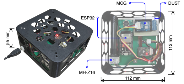
Fig. 2. Prototype of DALTON sensing device.
