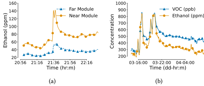
Fig. 19. Emitted pollutants such as – (a) Ethanol from fruit scraps in dining, (b) VOC and Ethanol from Food residuals and dirty dishes in the kitchen. It can be observed that the pollutants accumulate in the kitchen overnight and persist till the next day.
