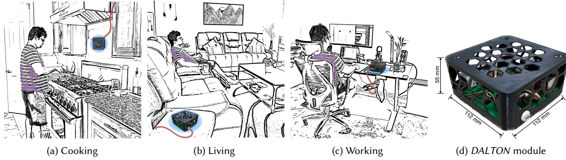
Fig. 1. DALTON platform in Household scenarios. We deployed multiple instances of the platform throughout different household rooms to capture the origin, spread, and spatiotemporal diversity of the indoor pollutants, providing better actionable insights.
