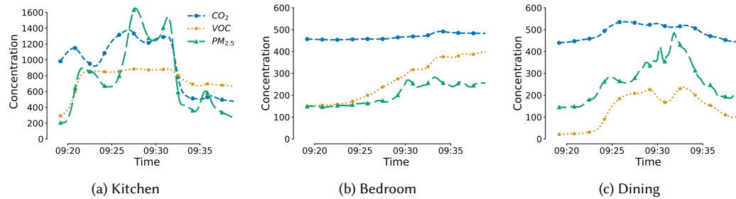
Fig. 14. The kitchen exhaust fan is off, while the dining ceiling fan of household H1 pulls the pollutants inward due to swirling airflow. Subsequently, it results in a worse spread where the kitchen (A), side by the bedroom (B), and dining (C) are all polluted.
