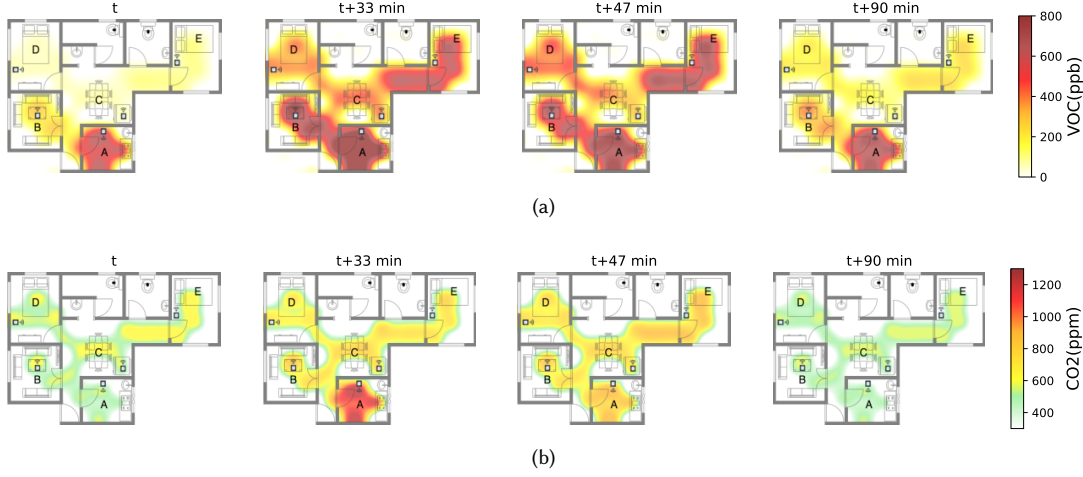
Fig. 17. Spatiotemporal spread of – (a) VOC, and (b) CO 2 from the kitchen (A) in Household H3. The cooking starts at t and ends at t+33 minutes. Both the pollutants get trapped in H3 due to the isolated room structure. CO 2 normalizes 57 minutes later at t+90 minutes when VOC persists in the kitchen (A) and the living room (B).
