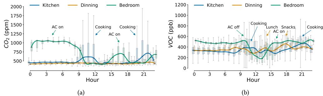
Fig. 18. Variations in concentrations of (a) CO 2 , and (b) VOC over hours of the day. Daily activities significantly influence the pollutants in the kitchen, dining room, and bedroom. For example, the bedroom gets polluted when the AC is on and the windows are closed. Similarly, the kitchen and dining area get polluted when food is prepared.
