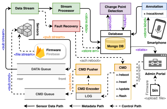
Fig. 3. IoT backbone microservices of DALTON platform. The solid arrow represents streaming data. The dotted arrow represents metadata such as data statistics, change points, etc. The dashed arrow represents error handling and control signals.
