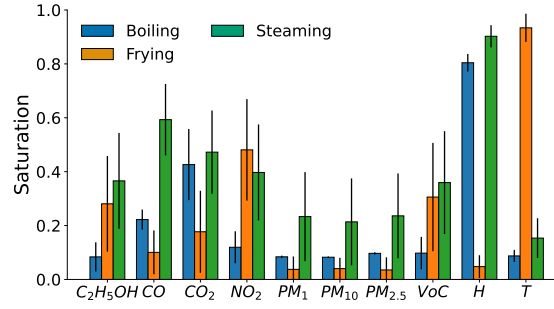
Fig. 20. Saturation of pollutants for different cooking methods. Boiling emits the least pollutants except CO and CO 2 from the burner. Frying increases temperature, so occupants turn on the exhaust fan, improving the ventilation. Steaming emits the most pollutants among the above cooking methods.
