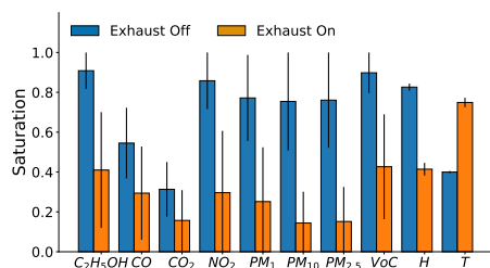
Fig. 10. Saturation levels of the pollutants with exhaust off vs on. Pollutants accumulate when the exhaust fan is off during cooking. Notably, the exhaust is turned on only at high temperature.
