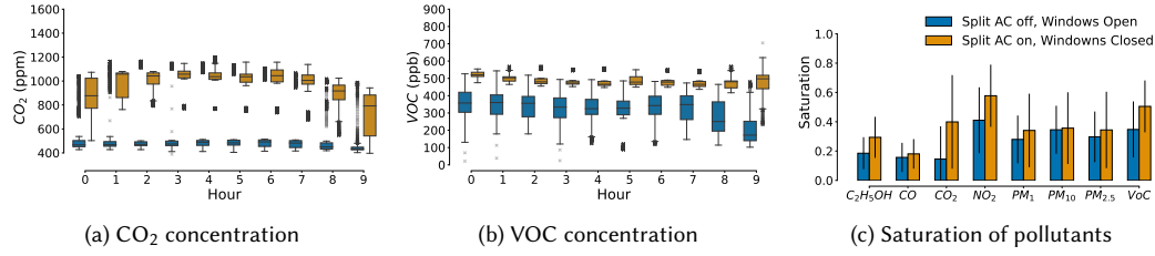
Fig. 8. Windows are closed for effective air conditioning using split AC. Thus, CO 2 and VOC accumulate dangerously over the night hours in summer when the split AC is running. Sub-figure (a) shows CO 2 concentration almost triples compared to when the windows are open. CO 2 gets ventilated in the morning when the windows are opened again. However, sub-figure (b) depicts VOC persists for a little longer. The degree of accumulation for other pollutants is shown in sub-figure (c).
