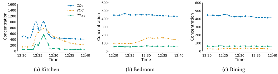
Fig. 13. The kitchen exhaust fan is on, dispersing most pollutants from household H1 to the outdoors. Therefore, the pollutants emitted during cooking in the kitchen (A) are effectively ventilated, and the other rooms remain largely unaffected.
