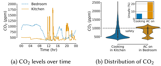
Fig. 9. In sub-figure (a), the kitchen shows sudden spikes of CO 2 while cooking. CO 2 accumulates in the bedroom while using split AC. On average, the bedroom is exposed to higher CO 2 concentration and 15.2% more unsafe than the kitchen, as per sub-figure (b).
